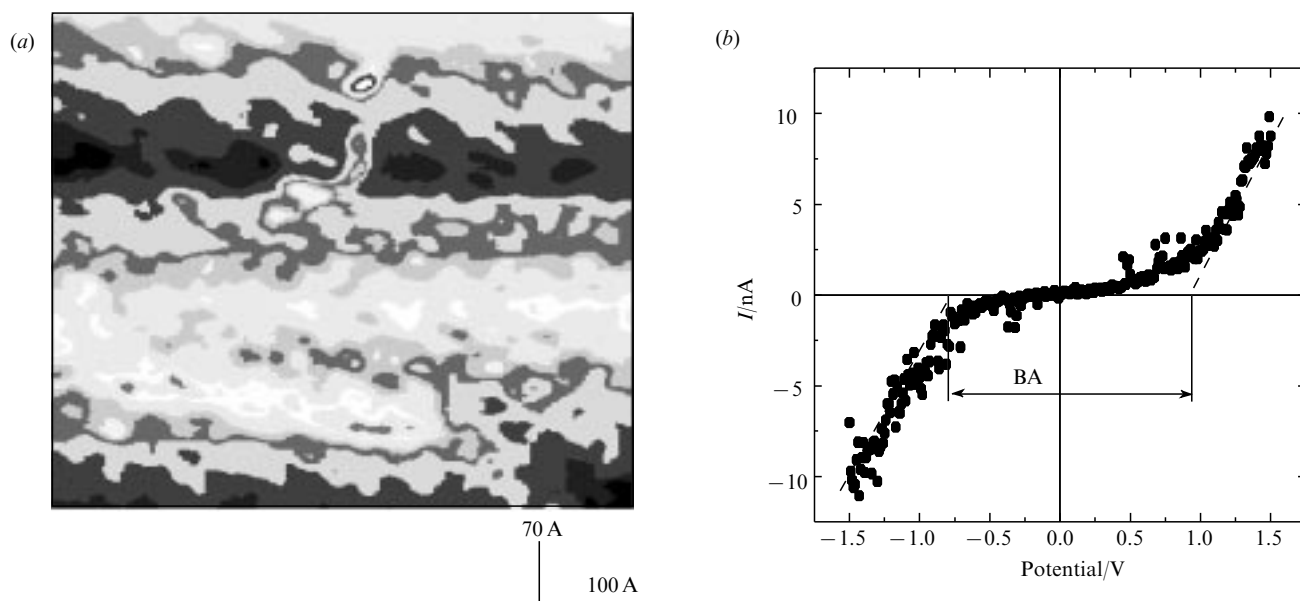
Figure 1 (a) Room temperature STM image of \text{Pd}_{10}(\text{CO})_{12}(\text{PBu}_3)_6 clusters deposited on a HOPG surface where single clusters can be observed. Arrows indicate the position of the tip during the CVC recording. (b) Tunnel characteristic CVC of the cluster; BA — the blockade area.
